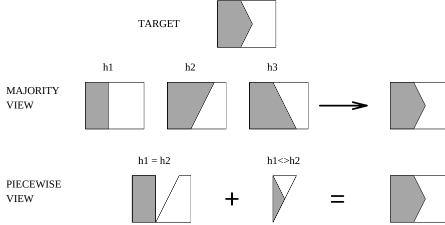
Figure 4.5: An alternative view of SBA. The SBA representation is commonly viewed as a majority of weak learners. An alternative view is of that of piecewise tiling of the domain. h_2 rejects the part of the domain on which it disagrees with h_1 . The rejected portion is classified by h_3 .
