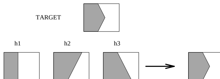
Figure 4.4: Boosting a weak representation. A linear separating classifier is too weak to represent the target concept shown above. However, a majority-vote ensemble of linear separators is able to represent this target. Most boosting algorithms build the ensemble incrementally. In this particular case three calls to the weak learner would return classifiers h_1 , h_2 , and h_3 in sequence.
