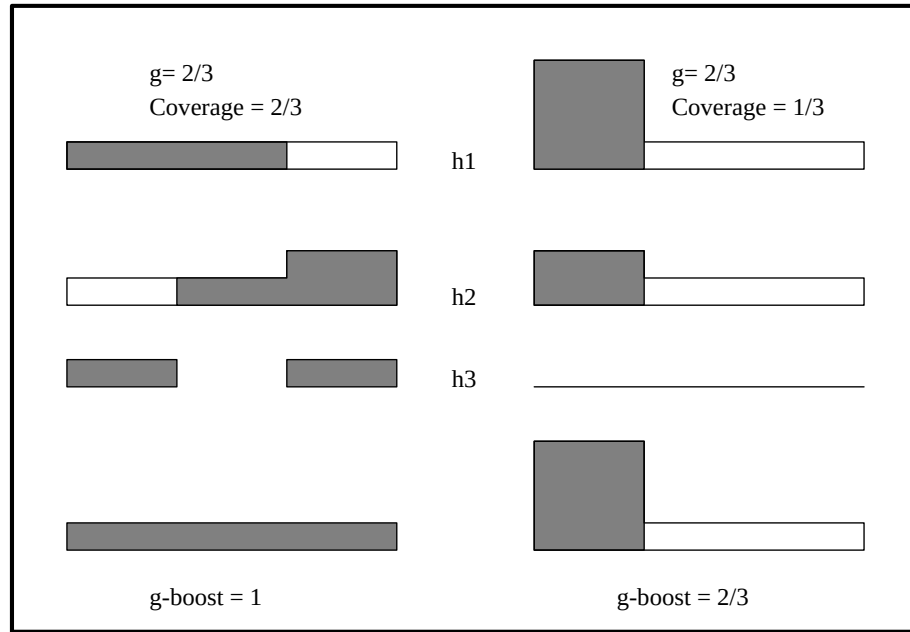
Figure 4.11: Boosting depends on fit. A pictorial depiction of the analysis in Section 4.3: in both the left and right examples the weak learner can produce a classifier with an accuracy of 2/3 . In the left example this is due to a reasonable fit of the target function. In the right example h_1 has a poor fit, but has the same accuracy due to the fact that the part of the domain covered by h_1 has a high probability density. The figure demonstrates the fact that boosting with SBA is dependent on the fit (or capacity) of the weak representation and not on the accuracy. This is particularly extreme in the right example which shows the case where \mathcal{D}_2 , the new training distribution for h , causes the generation of h_2 that is equivalent to h_1 and therefore no boosting occurs at all.
