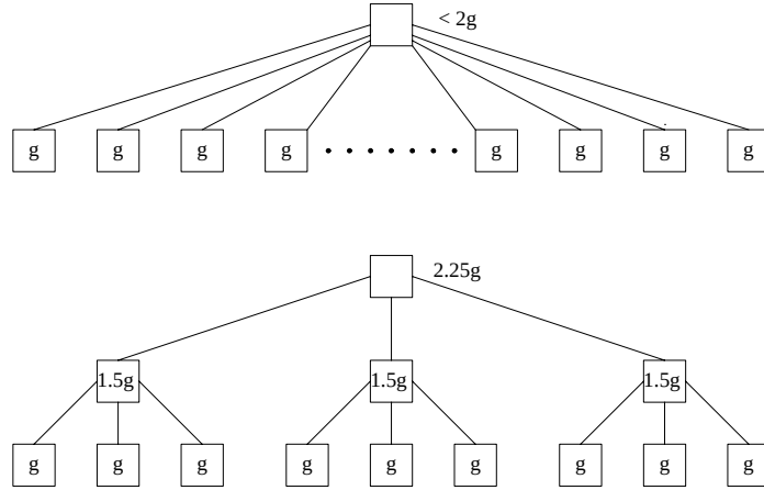
Figure 3.6: Hierarchical versus flat structures. Combining an arbitrary number of classifiers of accuracy g can give no more than accuracy 2g using a flat majority-vote classifier. However, using a hierarchical structure, 9 classifiers can be combined to achieve an accuracy of 2.25g .
