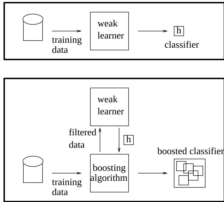
Figure 4.1: A boosting algorithm. The boosting algorithm uses a base-level weak learning algorithm as a black-box. The boosting uses the weak learner to generate classifiers from training data that is manipulated by the boosting algorithm. The boosting algorithm builds a new strong classifier using a combination of the classifiers returned by the weak learning algorithm.
