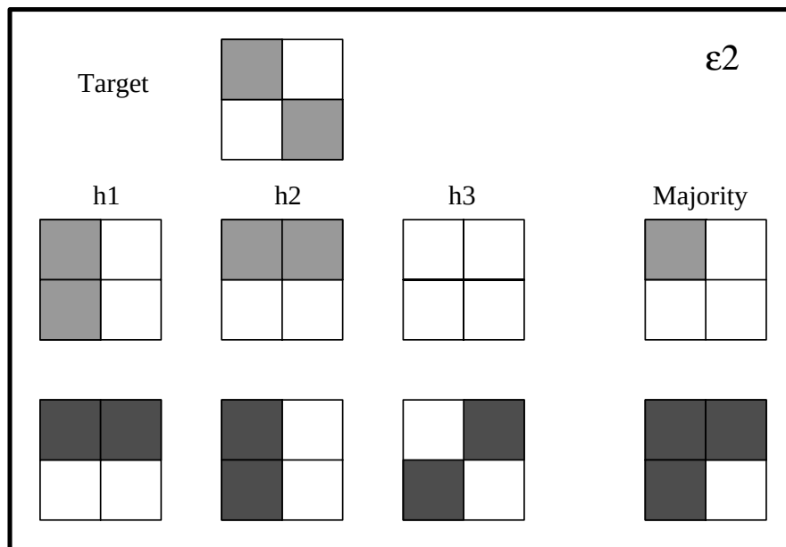
Figure 3.3: Ensemble \mathcal{E}_2 . A majority ensemble composed of classifiers performing at 50% correct. \mathcal{E}_2 's combined accuracy is 75% which is better than any individual in the ensemble. The bottom row plots the respective correctness indicator function.
