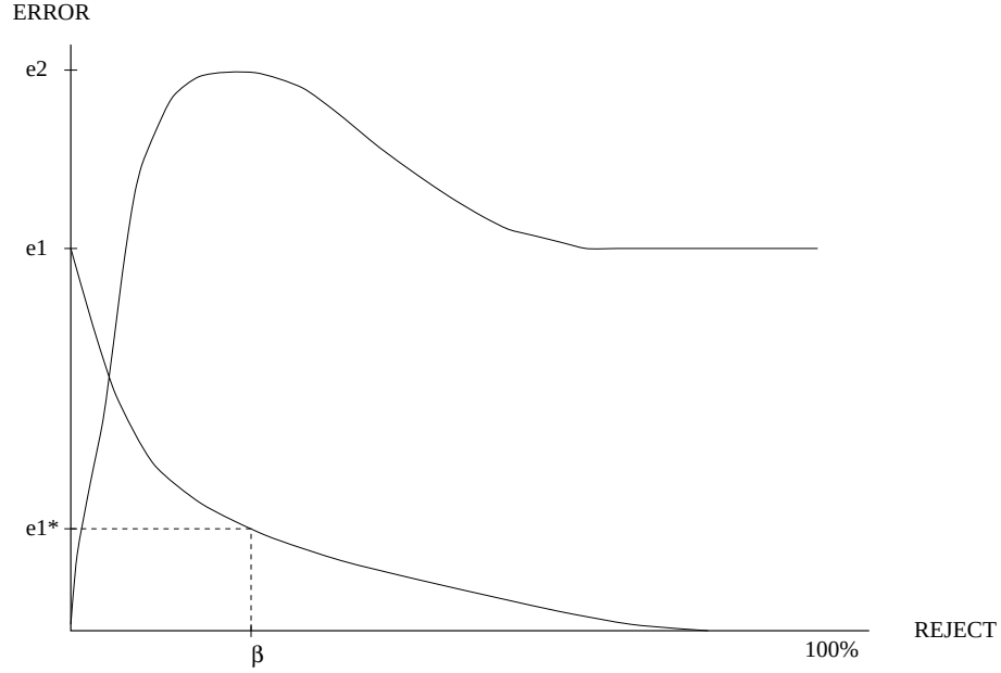
Figure 4.12: Schematics of the behavior of RBA as a function of \beta . The lower plot is the general form of the error rate \epsilon_{1R} as a function of the rejection rate. The second plot shows the typical behavior of \epsilon_2 , the error rate of h_{2R} as a function of the rejection rate \beta . When \beta is close to zero - very few patterns are rejected and h_{2R} can easily learn them. As \beta grows the distribution D_{2R} has a higher distribution of h_1 errors which makes the task for h_{2R} harder and we may expect a higher error rate. As \beta approaches 100%, the distribution D_{2R} becomes similar to the original distribution, and we expect \epsilon_2 to approach \epsilon_1 .
