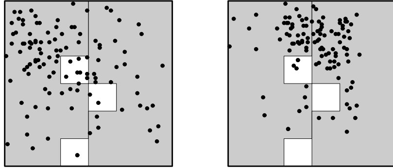
Figure 2.4: The accuracy depends on the pattern distribution. The same classifier can have different accuracies dependent on the distribution of patterns. The correctness indicator functions shown above are equivalent. However the classifier on the left will have lower accuracy since more instances “fall” into the white areas where it is incorrect.
