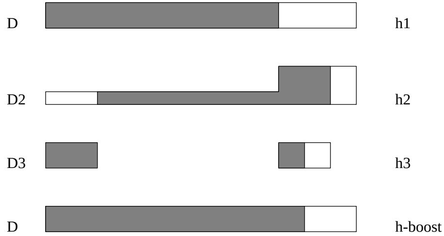
Figure 4.6: A pictorial description of Schapire's Boosting Algorithm. Each line depicts both the domain and a correctness indicator function for a classifier generated at a certain step. The whole domain is depicted as the points along the horizontal axis. The height at any point is proportional to the probability density function of the training distribution passed to the weak learner at that stage. We assume that the original distribution is uniform over the domain. The classifier h_1 only correctly classifies part of the domain and is trained on the original distribution D . The new training distribution D_2 is generated so that half of the patterns are h_1 errors and the other half are classified correctly by h_1 . Training on the new distribution will produce h_2 that will classify some of the patterns h_1 was unable to classify ( the "hard" patterns ) at the expense of erring on others that h_1 classified correctly. In step 3, D_3 includes only patterns on which h_1 and h_2 disagree. Since the areas which are not part of D_3 are "don't care", h_3 will be able to use some of its capacity on "hard" patterns. The resulting voting ensemble h_{boost} has higher accuracy than, h_1 , the original classifier the weak learner generated.
