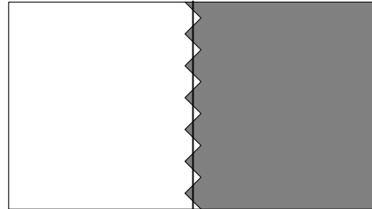
Figure 4.8: The zigzag concept may fit reasonably well by a linear separator, but boosting will cause only small increases in fit.
