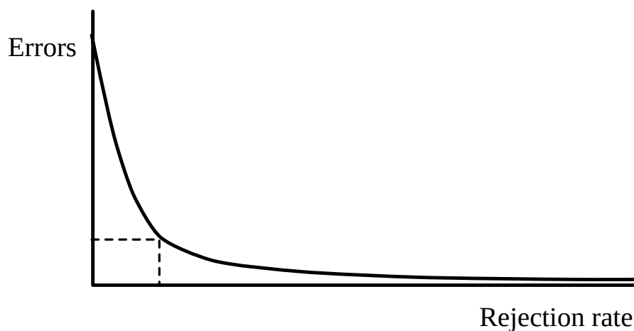
Figure 2.7: The typical form of error rate versus rejection rate. If the confidence score of a classifier is reliable, as one rejects more of the low confidence patterns, the number of errors among the accepted patterns will decrease. If we reject all patterns there are no errors, if no patterns are rejected, the error rate is just the raw error rate of Equation 2.6 often named the raw error rate .
