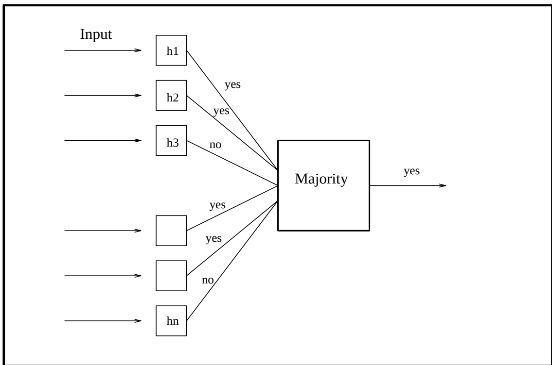
Figure 3.1: A majority-vote ensemble classifies by passing the input pattern to each of the individuals in the ensemble and choosing the class label according to a majority.
