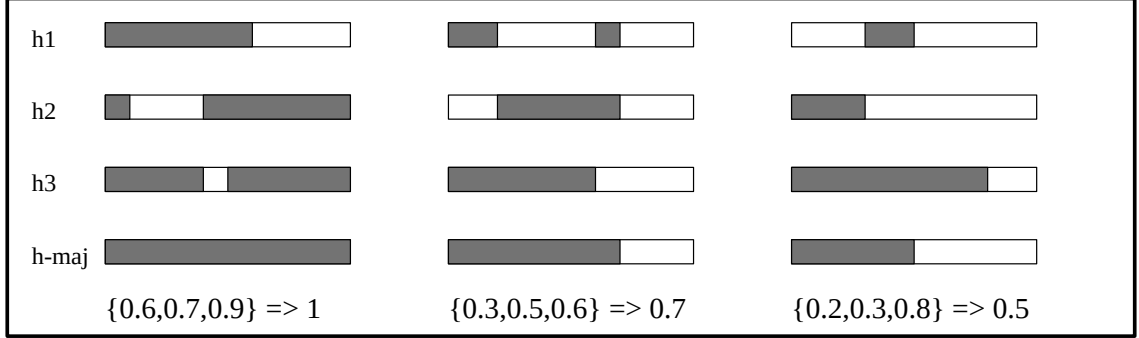
Figure 3.4: The upper bound on the accuracy for a 3-member ensemble. The three columns correspond to the three cases in Equation 3.27. Each column presents the correctness indicator functions of h_1, h_2 and h_3 to achieve a majority-vote ensemble with the highest accuracy possible with accuracies of g_1, g_2 , and g_3 . At the bottom of each column is a numeric example for each case. (1) The rightmost case occurs when the most accurate classifier has an accuracy greater than the sum of the other two. The upper bound in this case is just the sum of the two accuracies. (2) When the highest accuracy is smaller than the sum of the other two, it is possible to achieve an accuracy of half the sum of the accuracies (middle case) unless this value is greater than 1, which is the best one can achieve (leftmost case).
