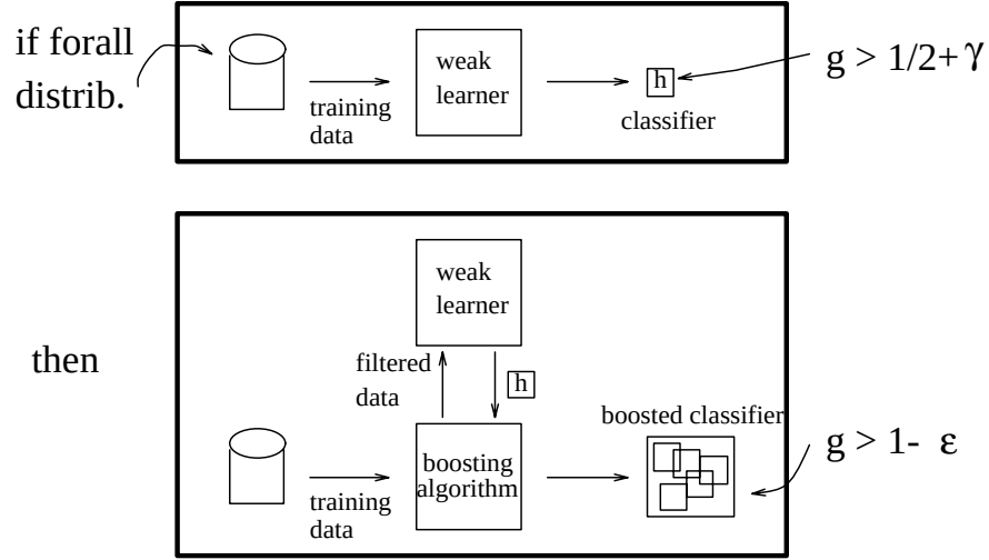
Figure 4.2: Theoretical qualities of boosting: if, for any training distribution, the weak learner is guaranteed to return a classifier that is better than 50% correct on the distribution it was trained on, then the boosting algorithm can return a classifier with an arbitrary level of accuracy.
