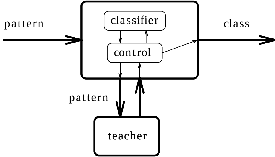
Figure 5.1: The on-site model.
