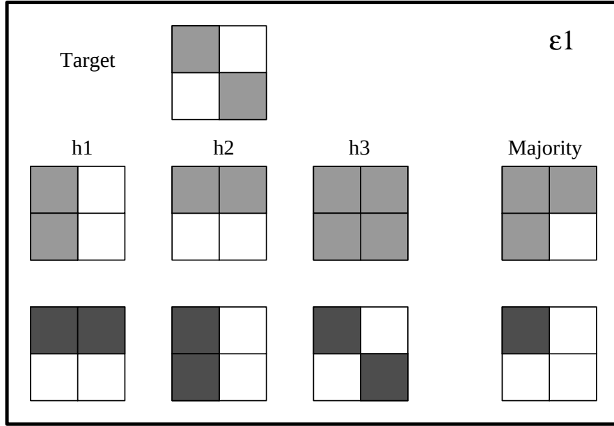
Figure 3.2: Ensemble \mathcal{E}_1 . A majority ensemble composed of classifiers performing at 50% correct. \mathcal{E}_1 's combined accuracy is 25% which is worse than any individual in the ensemble. The bottom row plots the respective correctness indicator function.
