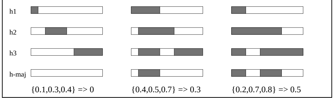
Figure 3.5: The lower bound on the accuracy for a 3-member ensemble. The three columns correspond to the three cases in Equation 3.29. Each column presents the correctness indicator functions of h_1, h_2 and h_3 to achieve h_2^3 with the lowest accuracy possible with accuracies of g_1, g_2 , and g_3 . At the bottom of each example are numeric examples for each case.
