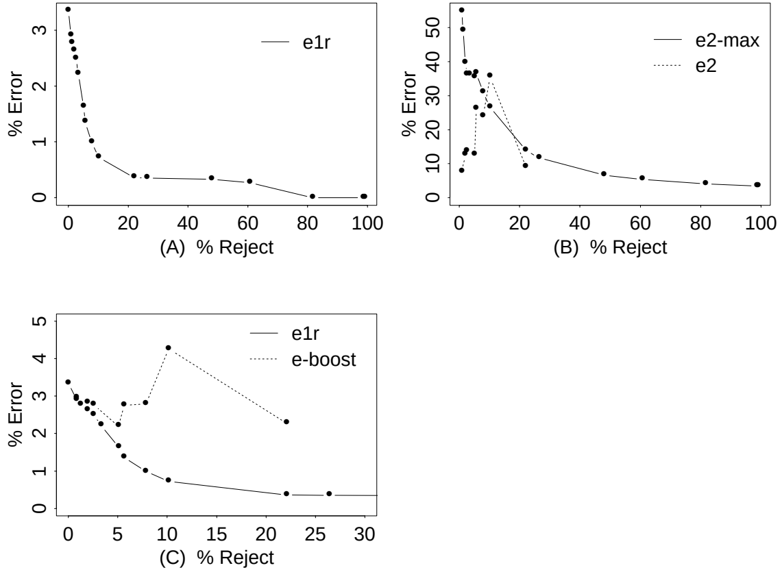
Figure 4.13: An example of the dependency of boosting on \beta . RBA give the ability to tune and possibly maximize the boosting. (A) Shows the empirical dependency of \epsilon_{1R} on \beta . (B) Using Equation 4.24 one can calculate \epsilon_2^{max} , the upper bound on the error of h_{2R} and compare it to the empirical value \epsilon_2 for various values of \beta . One can see that at approximately \beta = 15\% the error \epsilon_2 surpasses this bound. (C) At the point that \epsilon_2 surpassed \epsilon_2^{max} , RBA actually increases the error. At all other points there is a reduction in the error. One can experimentally search through the values of \beta to find the value that gives the best error reduction.
