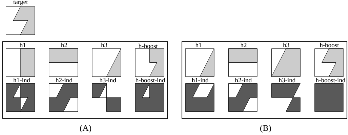
Figure 4.7: Results of applying SBA with a linear classifier as the weak learner in two different cases. The target concept is f(\{X, Y\}) = \Theta(Y \Leftrightarrow 2X + 1 \Leftrightarrow \Theta(Y)) where \{X, Y\} \in [\Leftrightarrow 1, 1]^2 and \Theta(w) \equiv [w \geq 0] is a step function. This example is simple enough to run SBA analytically. The purpose of the examples is to demonstrate that the boosting algorithm's success may depend on the initial concept ( h_1 ). In fact, a non-optimal fit for h_1 may give better overall results. Unless otherwise noted, the LM returns the best classifier it can fit for the distribution it is given. The top row gives the the three different concepts returned at each stage of the boosting algorithm and the final combined classifier. Directly below, the respective areas of the domain in error are shown. The error for h_3 is shown only for the part of the domain that is passed to the LM in step 3. (A): h_1 's accuracy is 87.5%, this is the optimal accuracy for a linear classifier for this target concept. h_2 's accuracy is 78.6% on D_2 and h_3 's accuracy on D_3 is 87.5%. The combined boosted accuracy is 93.75%. (B): For h_1 we choose a classifier whose accuracy is less than optimal (75%). The corresponding h_2 has an accuracy of 75% on D_2 and h_3 's accuracy D_3 is 100%. The combined boosted accuracy is 100%.
