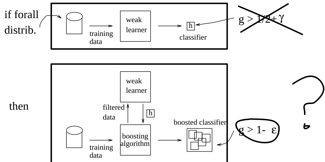
Figure 4.3: Boosting in practice. There are very few target concepts for which a weak learner is guaranteed, regardless of the distribution, to be better than chance. Therefore, a practical question is: will a boosting algorithm give a classifier that has superior accuracy and under what conditions?
