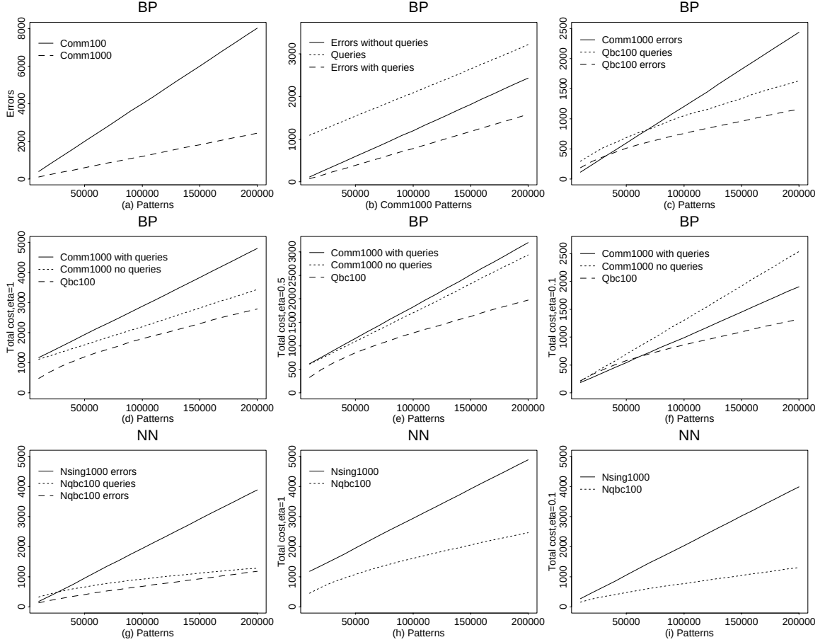
Figure 5.3: [Note the changes in scale] . Back-propagation (BP) and nearest neighbor (NN) runs trained on the concept 252a. (a) Demonstration of the simple fact that training on 1000 random patterns (Comm1000) gives better results than training on 100 random patterns (Comm100). (b) Comm1000 behavior with and without querying. (c) Raw results of BP runs. The error and query rates of Qbc100 decrease till they reach a constant. Also Qbc100's cumulative error drops below that of Comm1000 before it has made 500 queries. (d-f) Comparing the two different policies of Comm100 and that of Qbc100 for different values of \eta : \{1, 0.5, 0.1\} . One can see that as the cost of a query decreases, querying becomes more attractive even for the off-site network. (g) Raw results of NN runs. Nqbc100's query rate drops off very rapidly. (h-i) Total cost for NN with \eta = \{1, 0.1\} . The payoff for QBC seems more pronounced than in the feed forward networks.
