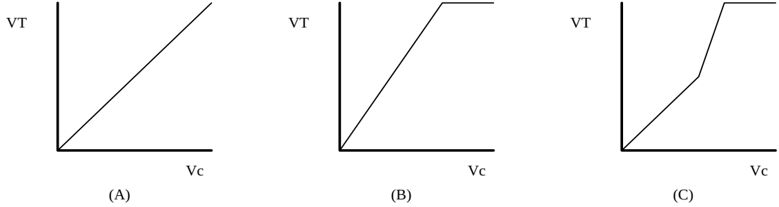
Figure 4.10: Comparison of V_T as a function of V_c : (A) No boosting is done. (B) Boosting using the optimal strategy to pick h_2 . (i.e. \Delta = V_c/2 ) (C) boosting using SBA. One can see that for V_c \geq 2/3 , SBA achieves 100% accuracy and for V_c < 1/2 , SBA does not boost at all. In the mid range 1/2 < V_c < 2/3 , SBA is sub-optimal and does not chose the best h_2 . [Axes are between 0 and 1.]
