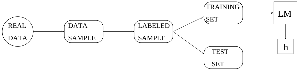
Figure 2.5: The methodology of building a classifier using machine learning. A corpus of data is sampled from the real world. The data is labeled with the “true” class label and divided to training and test data. A learning machine (LM) is applied to the training data and results in a classifier h . The classifier is tested using the test set. The accuracy on the test set is an estimate of the accuracy on the real world data (the “generalization” accuracy).
