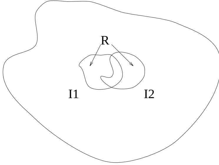
Figure 4.9: The rejection area. \mathcal{I}_1 is the area in domain that h_1 is correct. \mathcal{I}_2 is area where h_2 is correct. R is area where h_1 and h_2 disagree.
