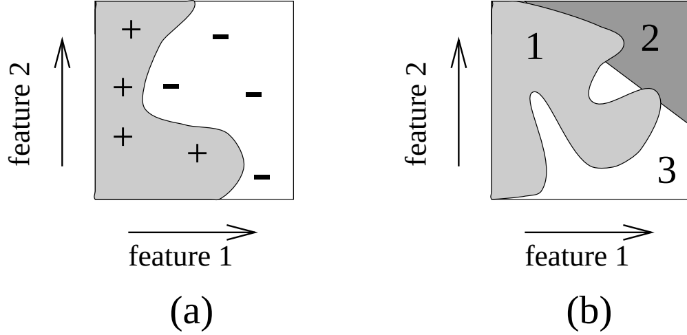
Figure 2.1: Target concepts. (a) A two-dimensional binary target concept. Positive instances are colored grey; negative instances are colored white. (b) A two dimensional ternary target concept.
